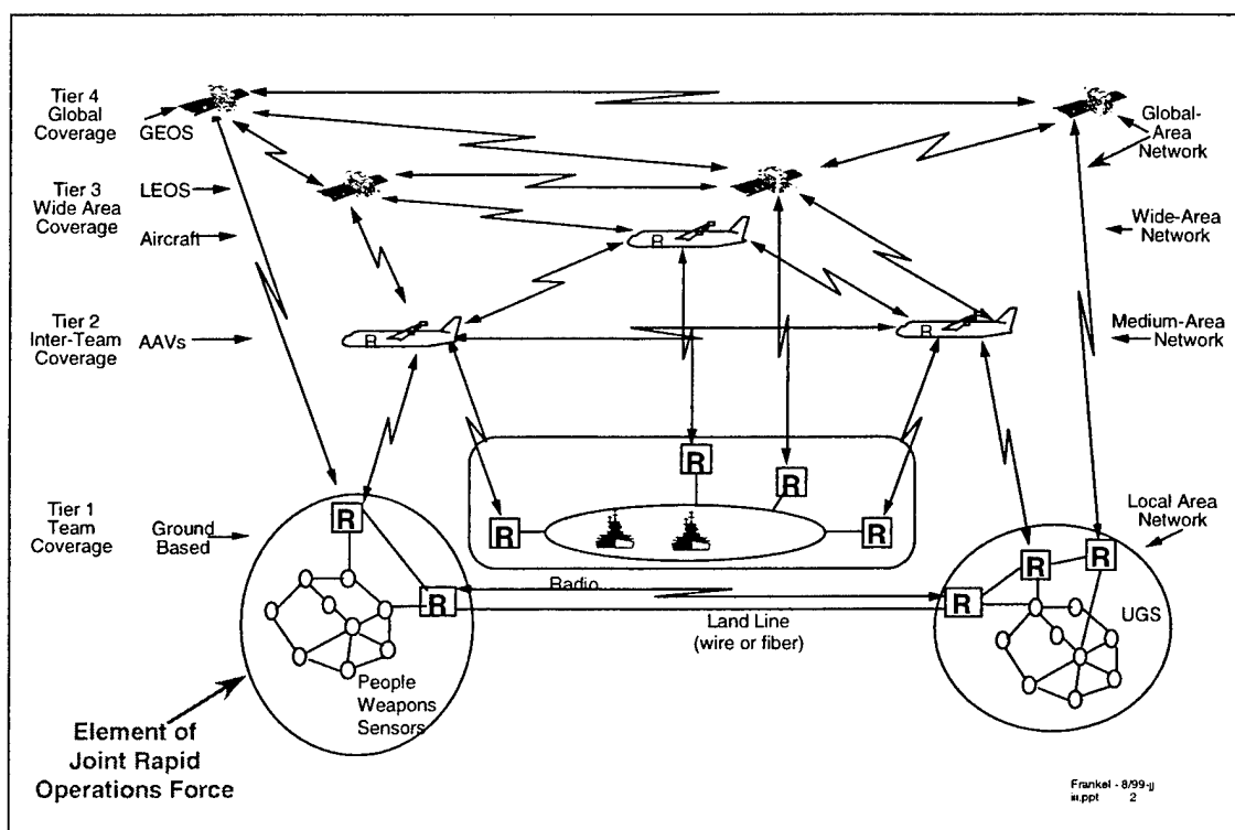
Figure 17. The Transport Layer of the Integrated Information Infrastructure
